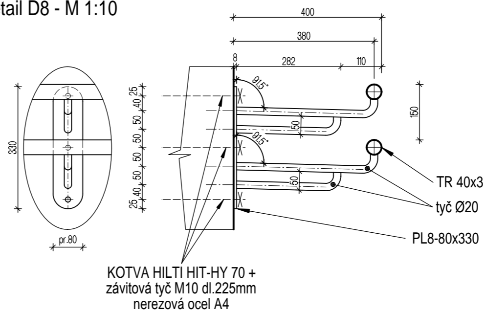
Detail D8 - M 1:10
