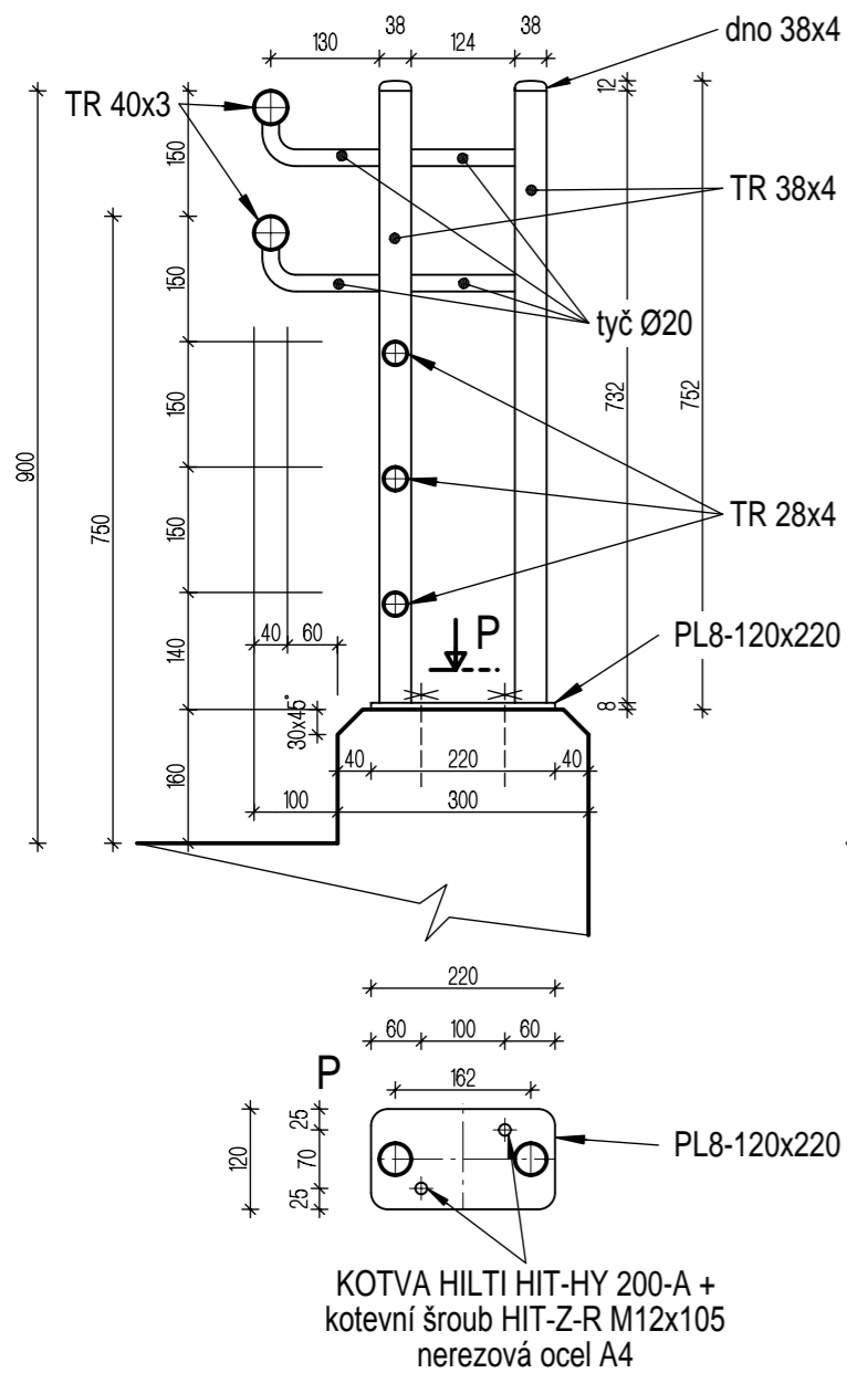
Detail D4 - M 1:10
